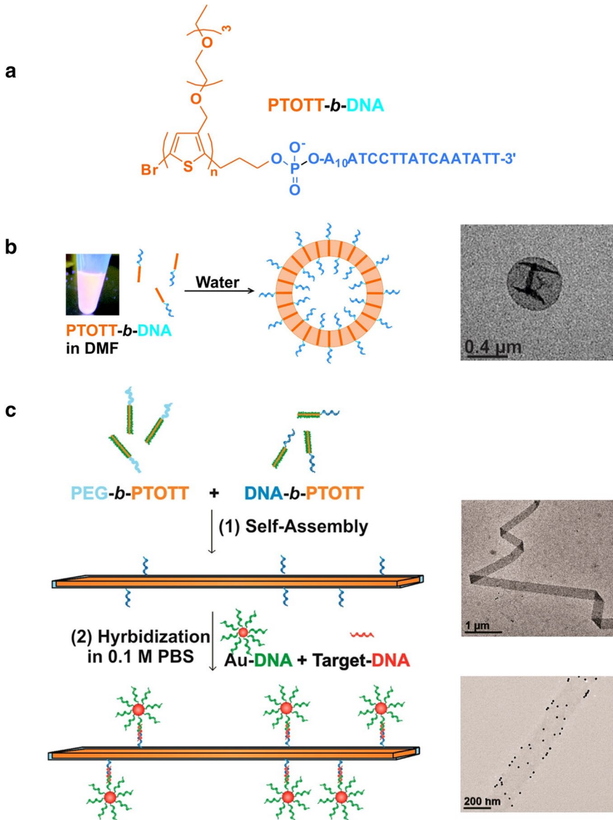
Fig. 19 a Chemical structure of ODN–PT conjugates. b ODN–PT conjugates self-assemble into vesicles in water; transmission electron microscopy (TEM) images of vesicles at the right. c ODN-b-PT conjugates can be co-assembled with PEG-b-PT to achieve the functionalization of the nanoribbons. TEM images at the right. Insets b , c are adapted with permission from [103]
